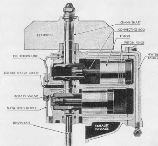
Cross section of twin cylinder, alternate firing, two-cycle engine showing points lubricated by the oil which is mixed with the gasoline.
