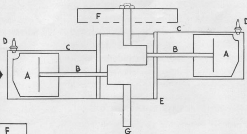
Twin cylinder opposed, two-cycle engine
