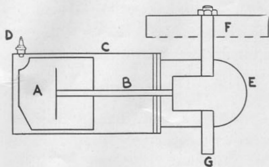
Single cylinder, two-cycle engine
