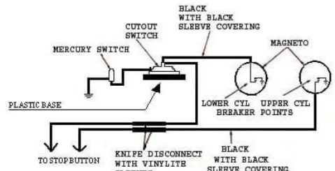
Kill Switch WIRING DIAGRAM FOR 1958-61 35 AND 40 HORSEPOWER MODELS (MANUAL START)
